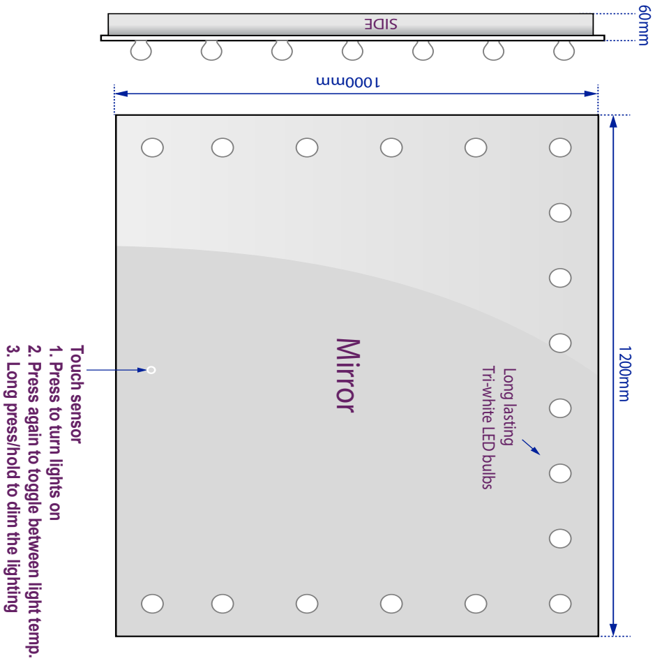
Views of complete assembly - With Mirror
