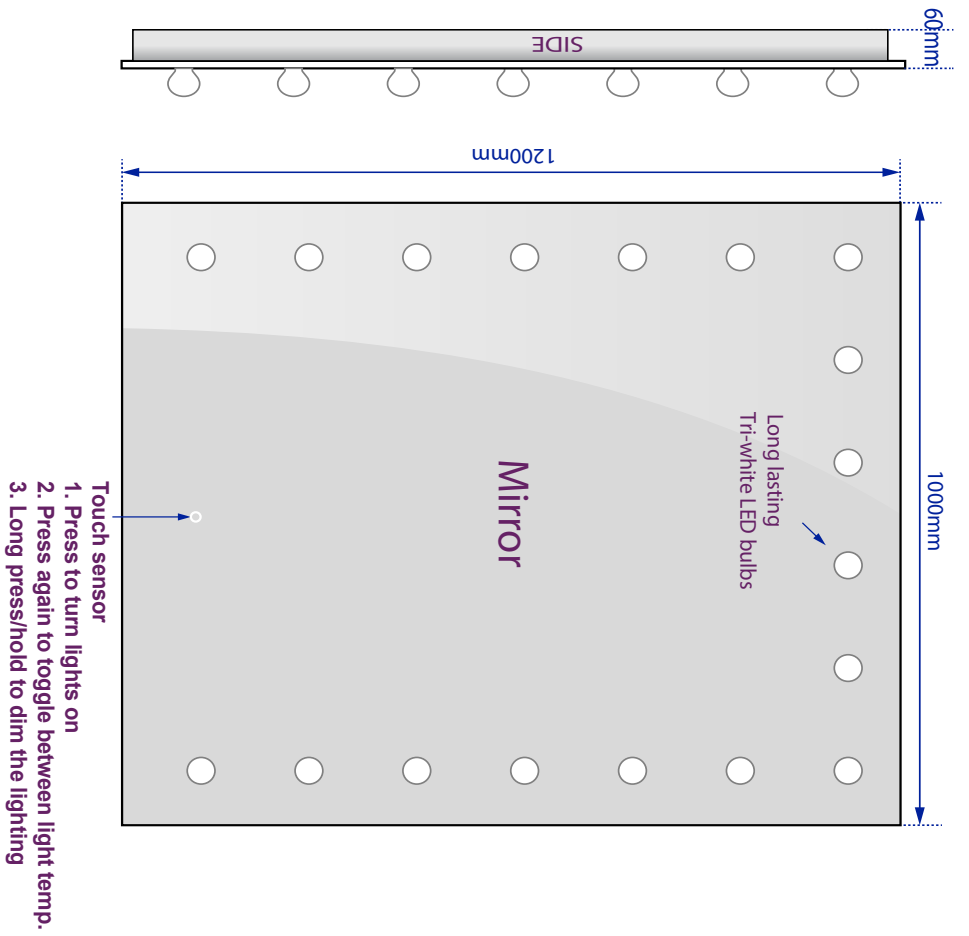
Views of complete assembly - With Mirror
